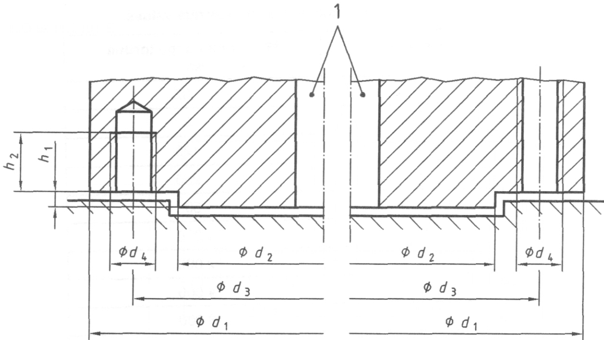
Figure 2 - Flange dimensions
